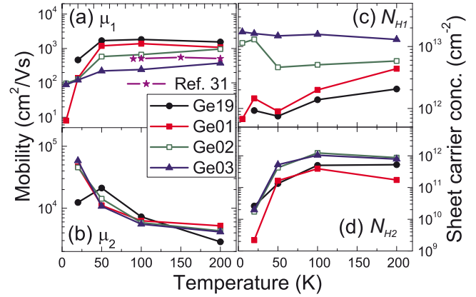
FIG. 3. (Color online) Fitting results of Hall curves at different temperatures. [(a) and (b)] Temperature dependent mobilities, data extracted from Ref. 31 is shown for comparison. [(c) and (d)] Temperature dependent sheet carrier concentrations. Lines are guides for eyes.
