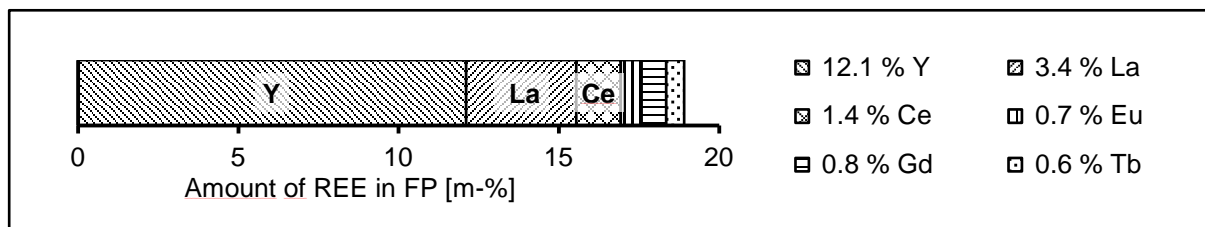
Fig.1: Elemental composition of the used FP measured by XRF in weight-%.
