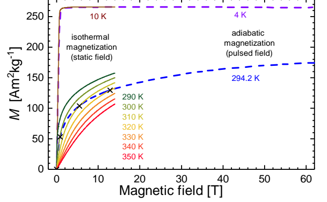
FIG. 4. Magnetization as a function of applied magnetic field. The solid lines represent isothermal measurements up to 14 T and the dashed curves were obtained in adiabatic pulsed-field experiments. Due to the large temperature increase during the pulse, the adiabatic curve strongly deviates from the isothermal results. Considering the adiabatic temperature changes in Fig. 2, it is possible to determine grid points (crosses) in order to match the pulsed-field data to the isothermally determined values of the magnetization.
