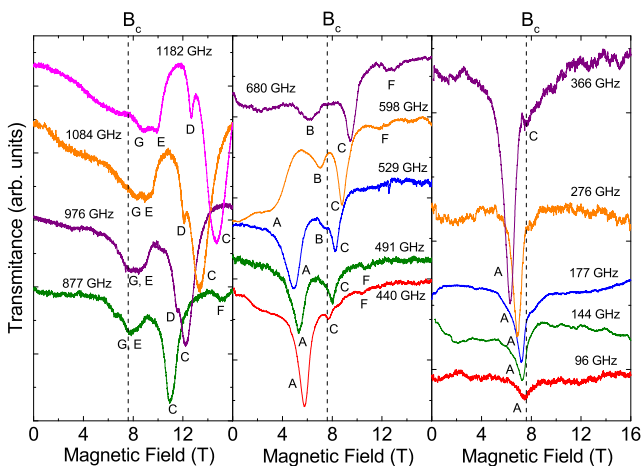
FIG. 3. Examples of unpolarized ESR spectra in \alpha -RuCl 3 for H \parallel [100] at various frequencies; T = 1.5 K. The spectra are normalized by the zero-field transmittance background and offset for clarity. The vertical line indicates the critical field as determined in Ref. [9].
