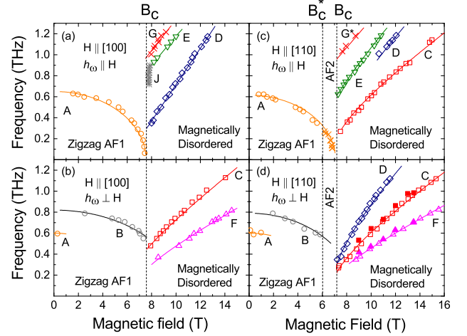
FIG. 2. Frequency-field dependences of magnetic excitations in \alpha -RuCl 3 for H \parallel [100] (a, b) and H \parallel [110] (c, d) ( h_\omega \parallel H (a, c), h_\omega \perp H (b, d), where h_\omega is the magnetic component of the THz radiation; T = 1.5 K). Absorptions denoted by crosses were observed using unpolarized radiation. Solid lines are guides to the eye. The vertical dashed lines indicate critical fields as determined in Ref. [9]. The closed squares and triangles in (d) denote inelastic neutron-scattering data from Ref. [10].
