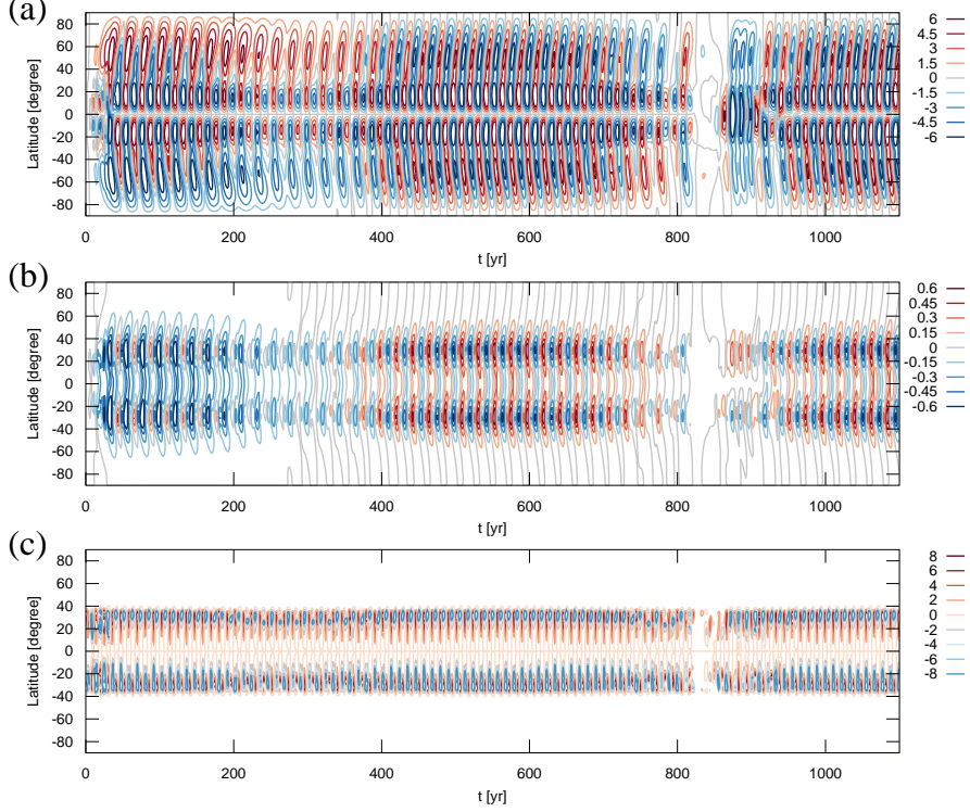
Figure 15. Behaviour of B(\theta, t) (a), A(\theta, t) (b), and \alpha(\theta, t) (c) showing transitions between dipole and quadrupole fields when varying \alpha_0^p according to \alpha_0^p(t) = 90(1 - 0.7 \sin^2(2\pi t/1100)) . The fixed parameters are \Omega_0 = 10000 , \alpha_0^c = 1 , \kappa = 1 , q_\alpha^p = 0.2 , q_\alpha^c = 0.8 .
