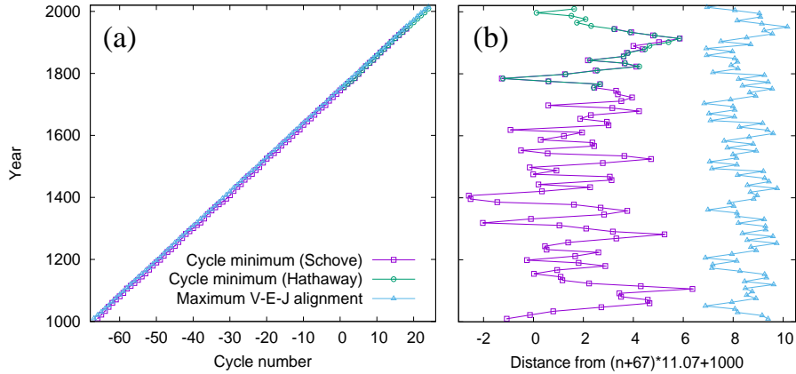
Figure 1. (a) Time series of the minima of the solar cycle according to Schöve (1955, 1983) and Hathaway (2010), and of the maximum alignment of the Venus-Earth-Jupiter system. (b) Deviation of the time series from a linear function f(n) = 11.07(n + 67) + 1000 of the cycle number n .
