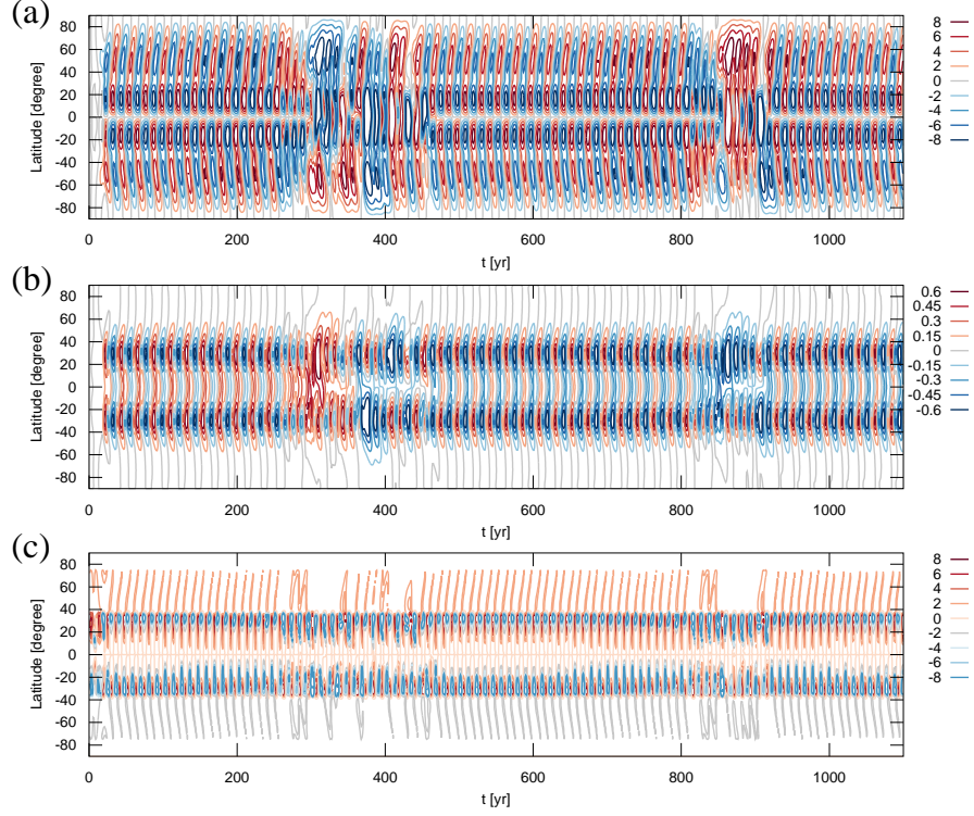
Figure 16. Behaviour of B(\theta, t) (a), A(\theta, t) (b), and \alpha(\theta, t) (c) showing transitions between dipole and quadrupole fields when varying \kappa according to \kappa(t) = 1(1 - 0.6 \sin^2(2\pi t/1100)) . The fixed parameters are \Omega_0 = 10000 , \alpha_0^c = 4 , \alpha_0^p(t) = 100 , q_\alpha^p = 0.2 , q_\alpha^c = 0.8 .
