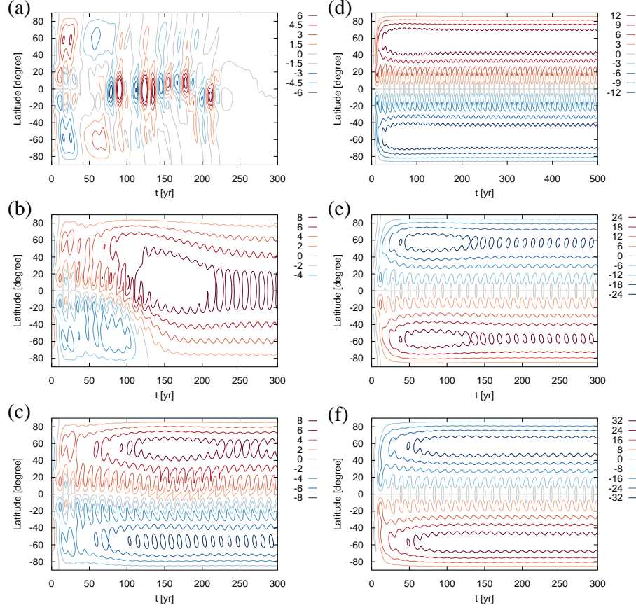
Figure 3. Behaviour of B(\theta, t) of the synchronized Tayler-Spruit dynamo with a nearly pure periodic \alpha^p term. The fixed parameters are \omega_0 = 10000 , \kappa = 0 , \alpha_0^c = 0.001 , q_\alpha^p = 0.2 , the initial conditions are s = 3 and u = 0.001 , and the varying parameter is \alpha_0^p = 16.1 (a), 16.2 (b), 16.3 (c), 30 (d), 70 (e), 150 (f). Note that, here and throughout the paper, the ordinate axis represents not the co-latitude \theta but the normal solar latitude 90^\circ - \theta .
