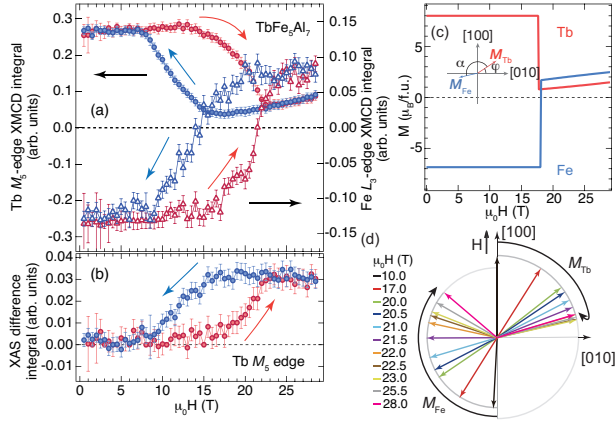
FIG. 6: Field dependence of (a) the integrated Tb M_5 -edge (left) and Fe L_3 -edge (right) XMCD signal and (b) the integrated Tb M_5 -edge XAS difference at 50 K. The sign of the integrated XMCD signal in panel (a) is reversed as in Figs. 1(c) and (d). (c) Tb 4f ( M_{Tb} ) and Fe 3d ( M_{Fe} ) moment as function of magnetic field simulated by the two-sublattice model. The inset shows the canting angles used in the simulation (see text for details). (d) Schematic diagram of the sublattice-moment rotation in magnetic field estimated from the data in (a) and (b) during the field up-sweep. The black arrows show the rotation direction on increasing magnetic fields.
