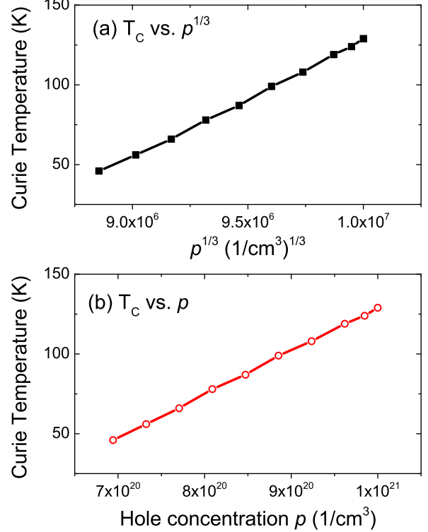
FIG. 10. Curie temperature vs. hole concentration p : (a) p^{1/3} and (b) p for samples Mn6ann_0, 9. The hole concentration is estimated by following the approach in Ref. 40.
