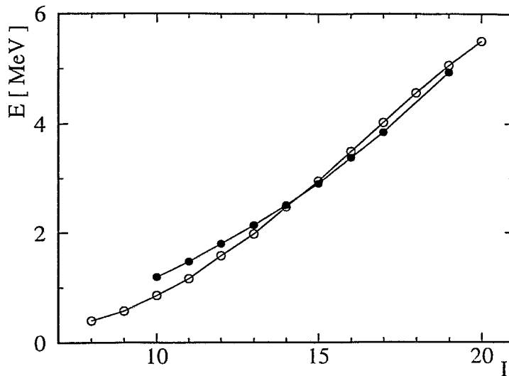
Fig. 9. Energy of the two lowest bands of positive parity in ^{134}\text{Pm} . The data is from ref. [15], where band 1 (full dots) is assigned to the configuration of a h_{11/2} quasi proton combined with a h_{11/2} quasi neutron.
