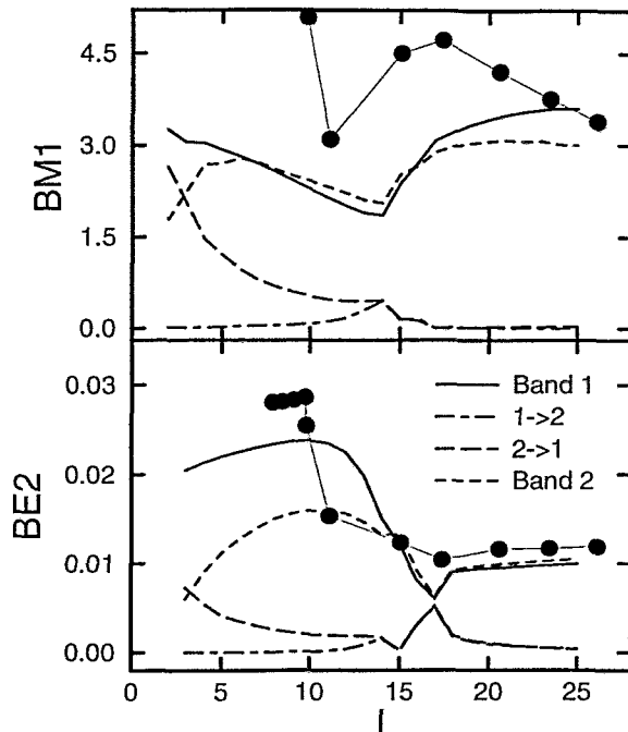
Fig. 7. BM1 and BE2 values from the particle rotor calculation for the case of a proton and a neutron hole coupled to the triaxial rotor.
