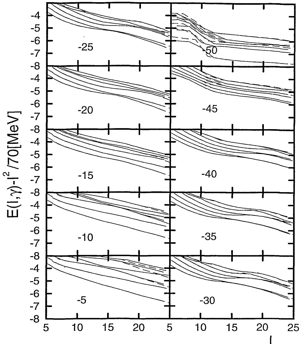
Fig. 8. Rotational levels of a h_{11/2} proton and a h_{11/2} neutron hole coupled to a triaxial rotor with different values of \gamma , which are indicated by the numbers in the panels. Full lines correspond to even and dashed to odd spin.
