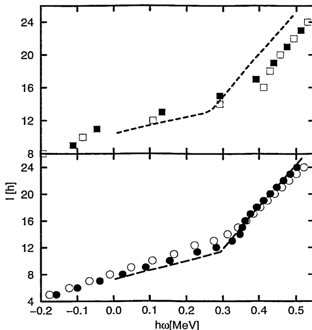
Fig. 4. The functions I(\omega) for h_{11/2} particles and holes coupled to a triaxial rotor with \gamma = -30^\circ . The upper panel shows the case of a proton and a neutron hole and the lower panel the case of a proton particle and a neutron hole. The frequency is calculated by means of \omega(I) = (E(I+1) - E(I-1))/2 from the PRM energies in fig. 2. In the upper panel the full squares are obtained from the odd spin yrast levels and the open squares from the even spin yrast levels. In the lower panel the open circles are obtained from the yrast band (both signatures) and the full circles from the yrare band (both signatures). Dashed lines correspond to the TAC calculations, where I = J - 1/2 is shown. For a discussion of the quantal correction 1/2 , cf. ref. [9].
