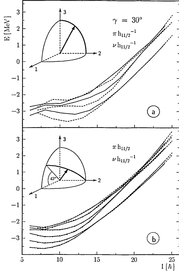
Fig. 2. Rotational levels of h_{11/2} particles and holes coupled to a triaxial rotor with \gamma = -30^\circ . The upper panel shows the case of a proton and a neutron hole and the lower panel the case of a proton particle and a neutron hole. Full lines correspond to even and dashed to odd spin.
