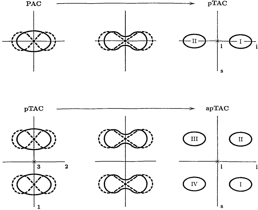
Fig. 5. Localization of the wave functions for PAC, planar TAC (pTAC) and aplanar TAC (apTAC) solutions. The full drawn ellipses symbolize the lowest solution at each position, which is symmetric. The dashed curves symbolize the first excited solution, which is odd.
