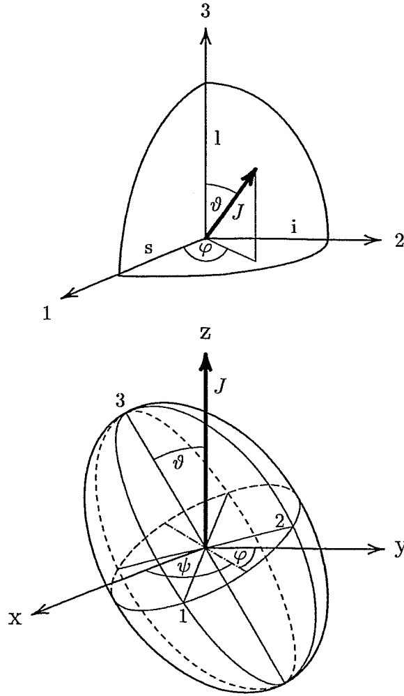
Fig. 1. Orientation of the axis of rotation ( J , displayed as the heavy vector) with respect to the principal axes of the triaxial density distribution (upper panel) and orientation of the triaxial density distribution in the lab. frame (lower panel). The long, intermediate and short semi axes of the density distribution are labeled by l , i and s , respectively.
