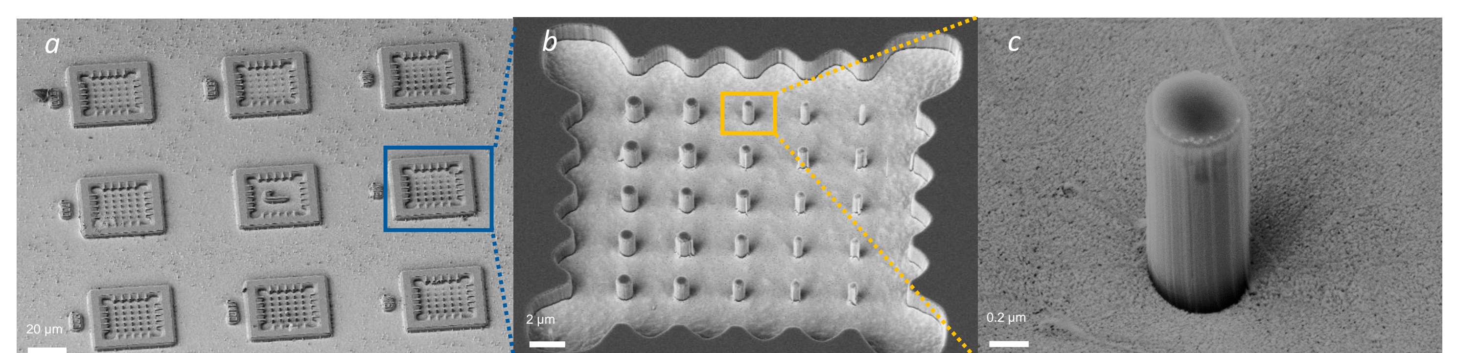
Fig. 6 SEM micrographs a) group of arrays and b) a single array of pillars with varying diameters, c) a single pillar ( \varnothing 600 \text{ nm} )
