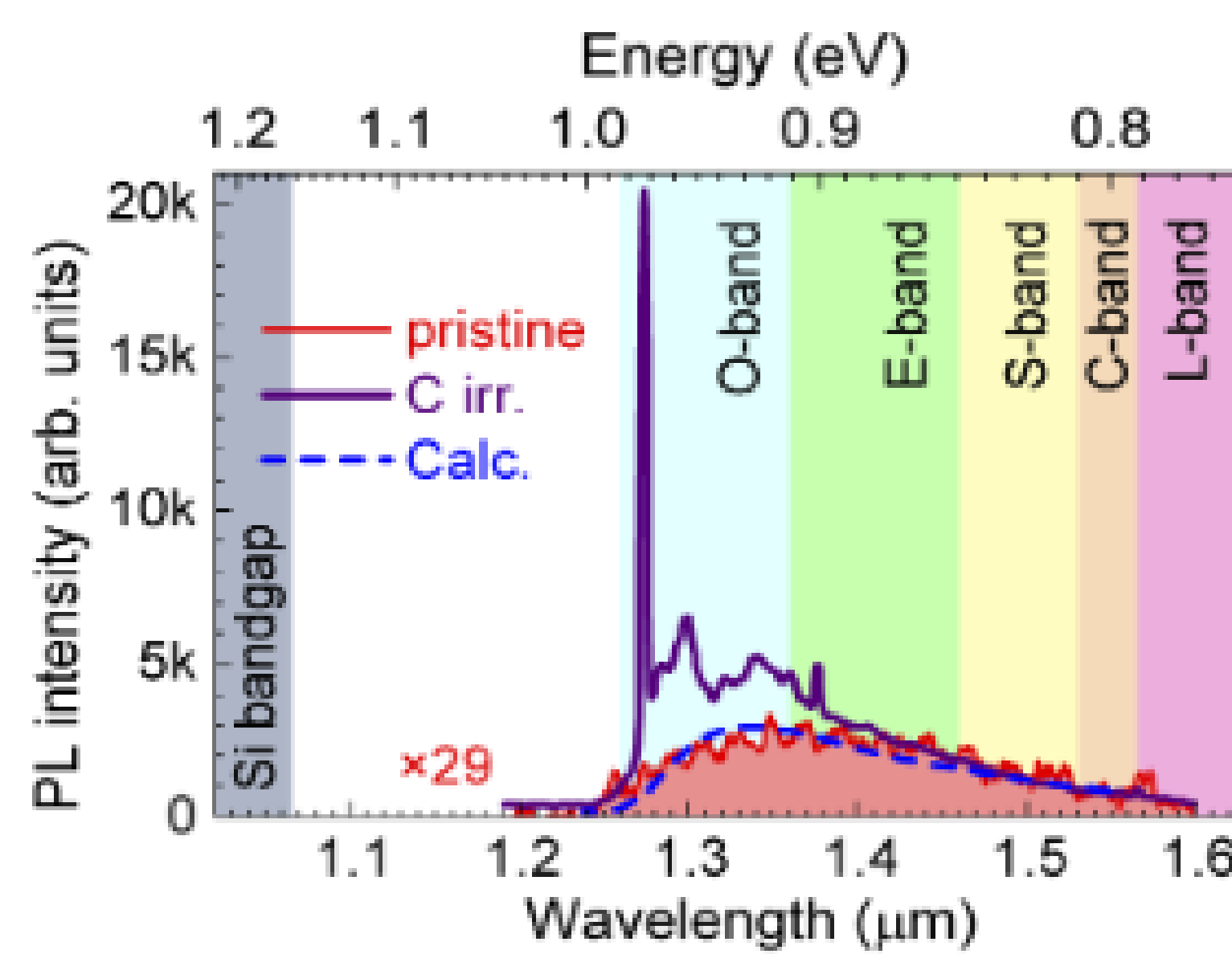
Fig. 3 Optical properties of G centers [1]
